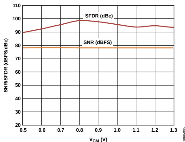
Figure 46. SNR/SFDR vs. Common-Mode Voltage ( V_{CM} ), f_{IN} = 9.7 MHz, f_{SAMPLE} = 125 MSPS, V_{REF} = 1.0 V
