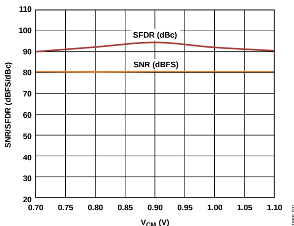
Figure 47. SNR/SFDR vs. Common-Mode Voltage ( V_{CM} ), f_{IN} = 9.7 MHz, f_{SAMPLE} = 125 MSPS, V_{REF} = 1.4 V
