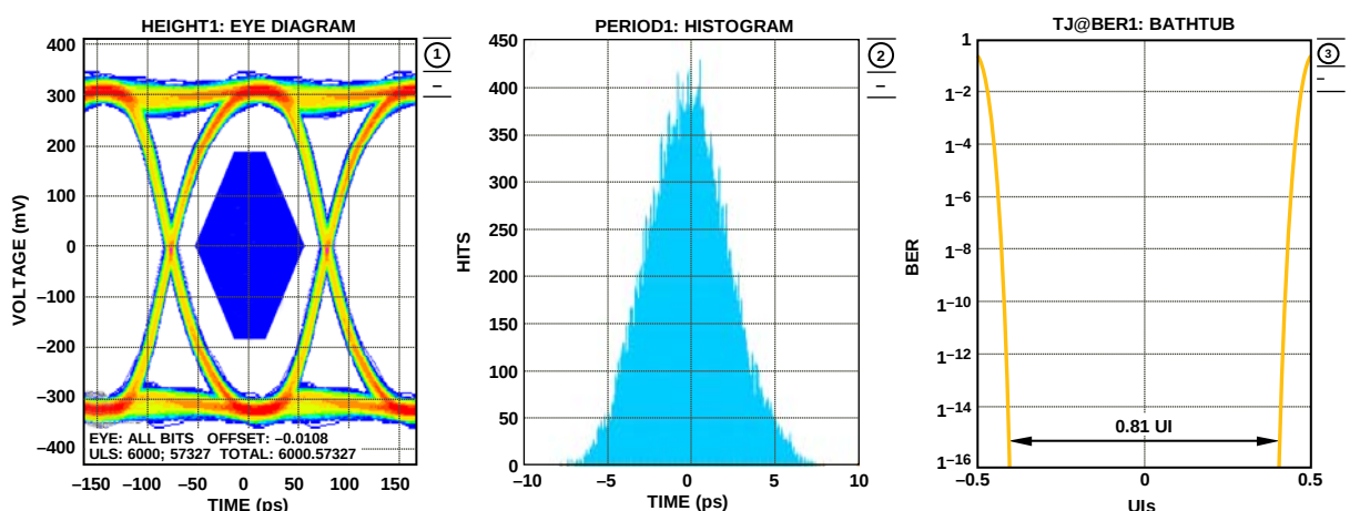
Figure 69. AD9656 Digital Outputs Data Eye, Histogram, and Bathtub, External 100 \Omega Terminations at 6.4 Gbps
