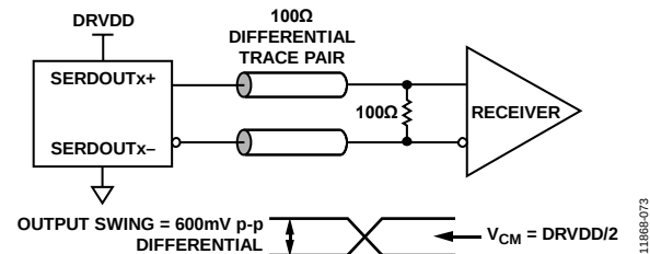
Figure 68. DC-Coupled Digital Output Termination Example
